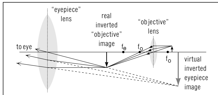
Figure 6. Image formation in a two-lens (“compound”) microscope. The focal length for the objective lens is f_o ; for the eyepiece lens, f_e .
